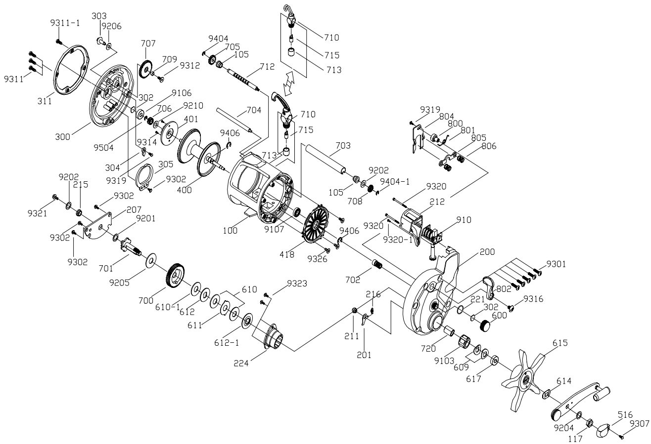
CN - 30D Spare Parts
